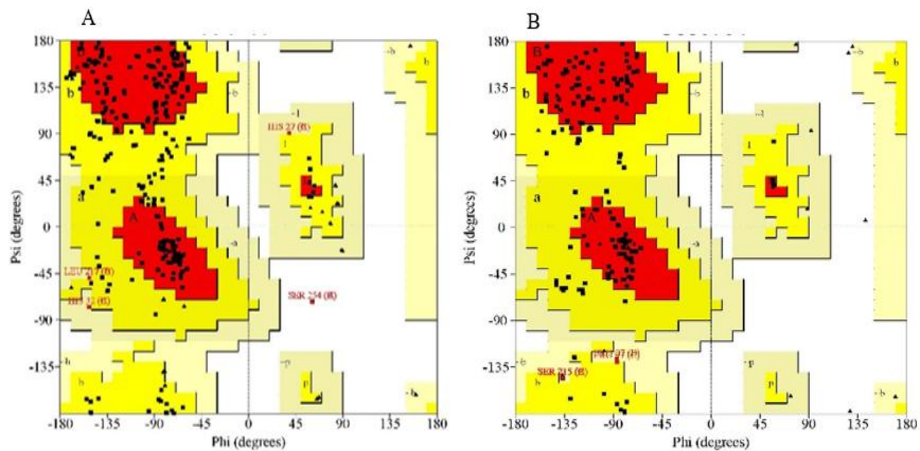
Supplementary Figure 1. Ramachandra plots of geometry minimized glutelin type-B 5-like protein models (A) model from Swiss-Model server (B) model from Robetta server.
