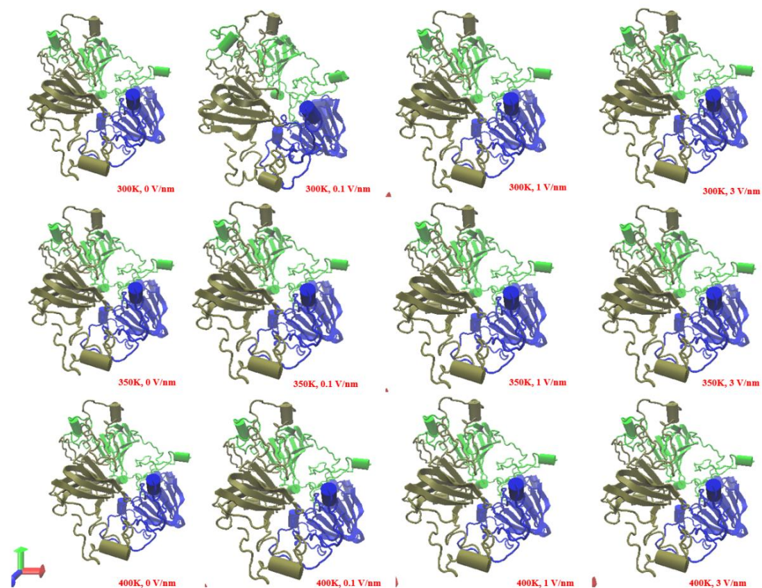
Supplementary Figure 2. Snapshots of glutelin type-B 5-like protein molecule after 1 ns simulation under different simulation conditions. No major disruption to the secondary structure. No difference observed in the snapshot.
