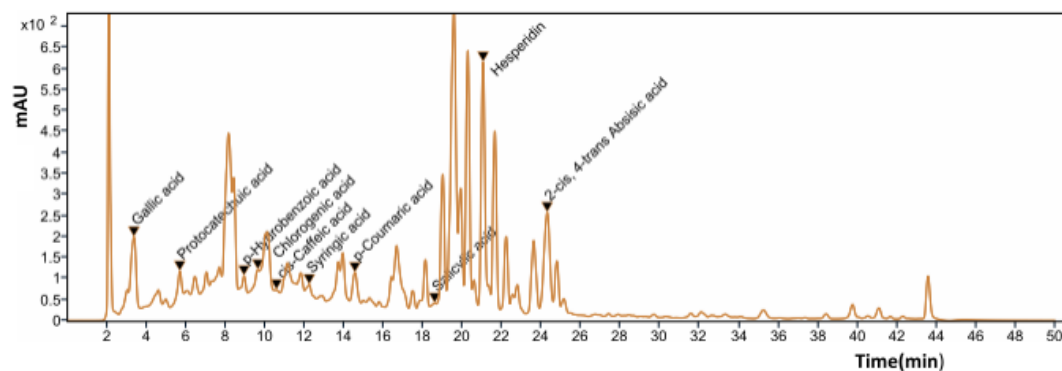
Supplemental Figure 1. Typical chromatogram of Psidium guajava leaves aqueous extract at 273 nm
