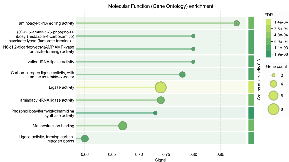
Figure S1. Predicted molecular functions of guaB -encoded PPINs based on GO terms.
