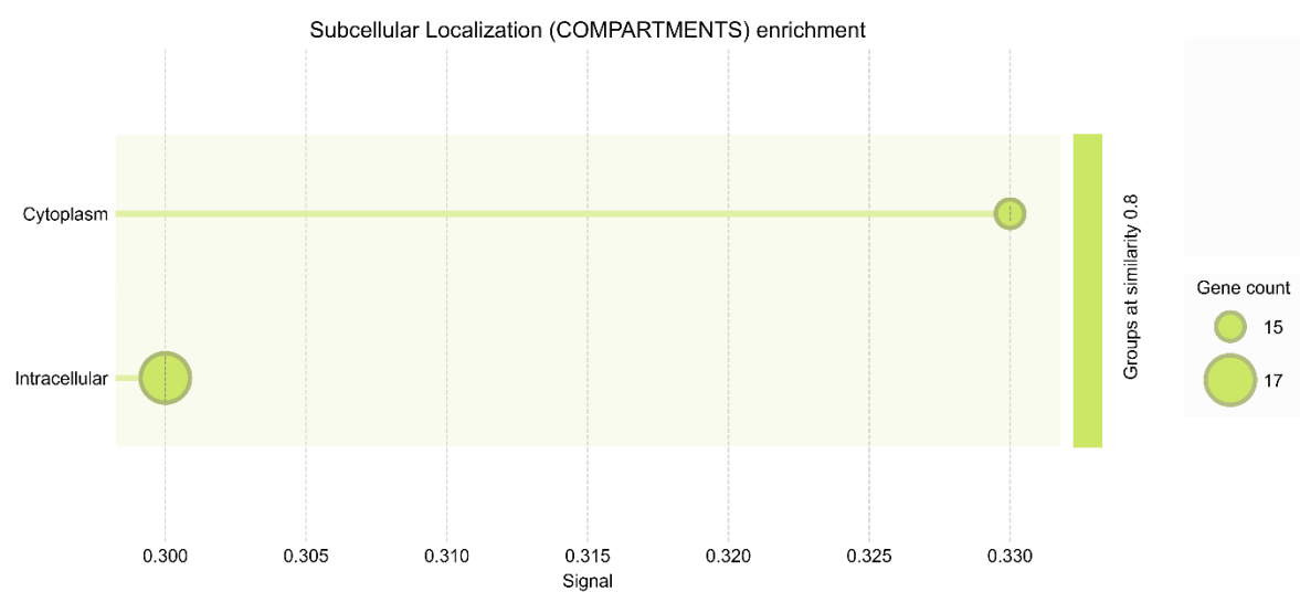
Figure S2. Predicted cellular components of guaB -encoded PPINs.
