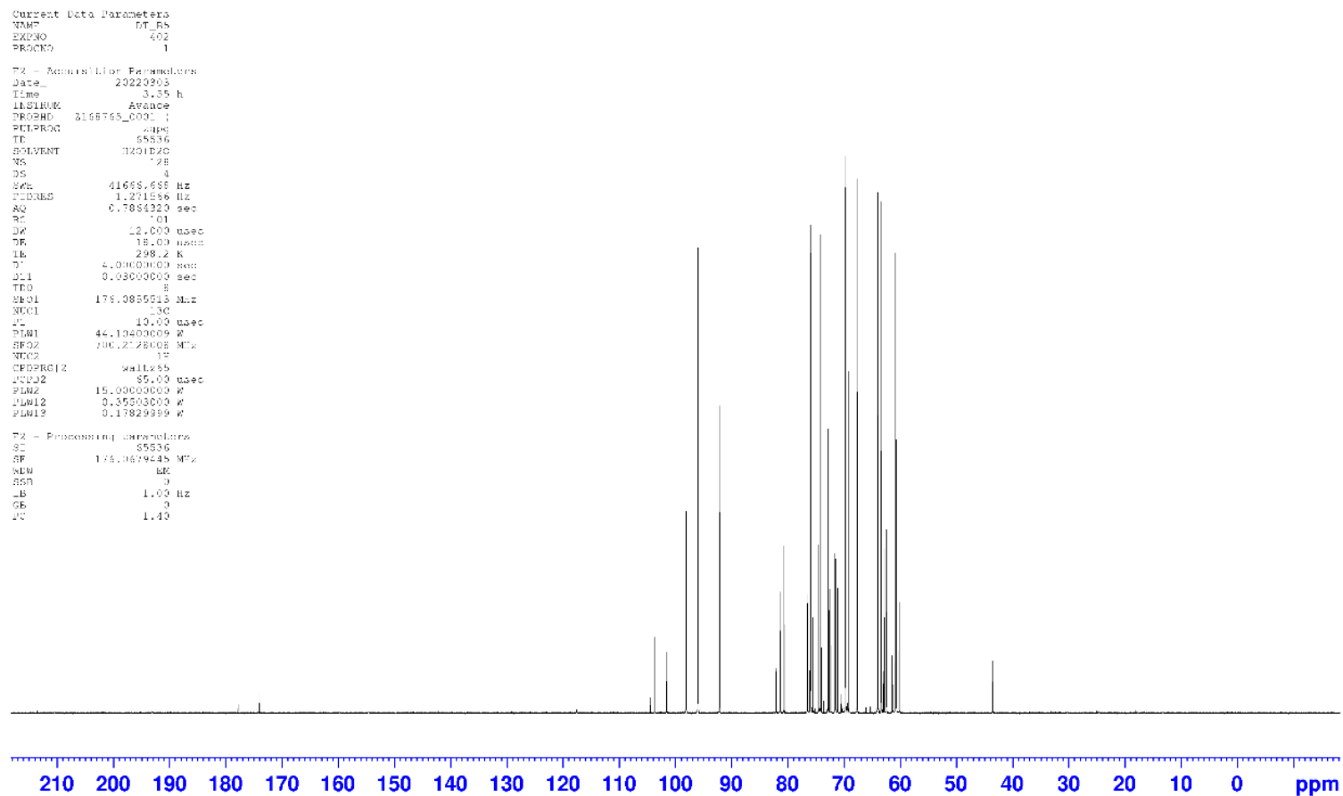
Figure S12 13 C-NMR Fingerprint
