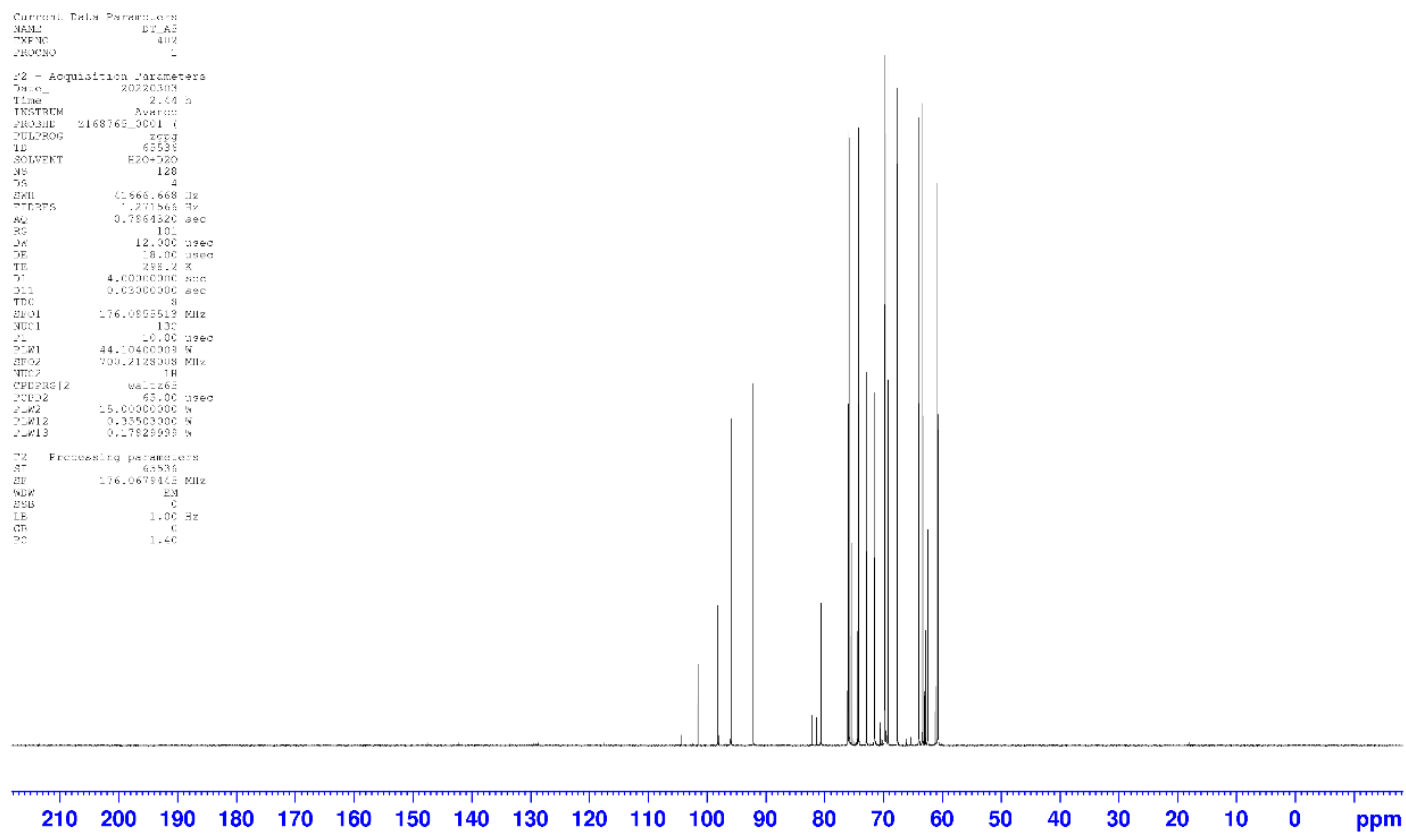
Figure S5 13 C-NMR Fingerprint
