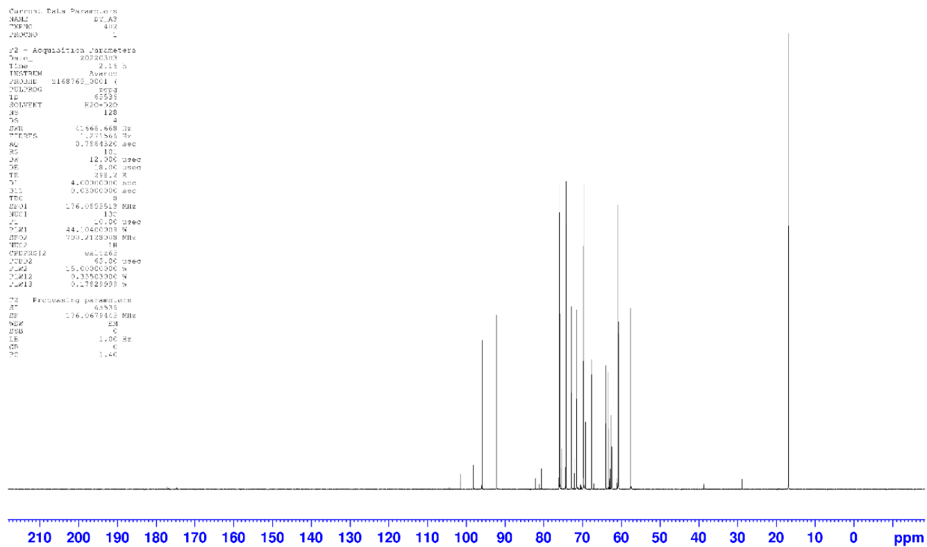
Figure S3 13 C-NMR Fingerprint
