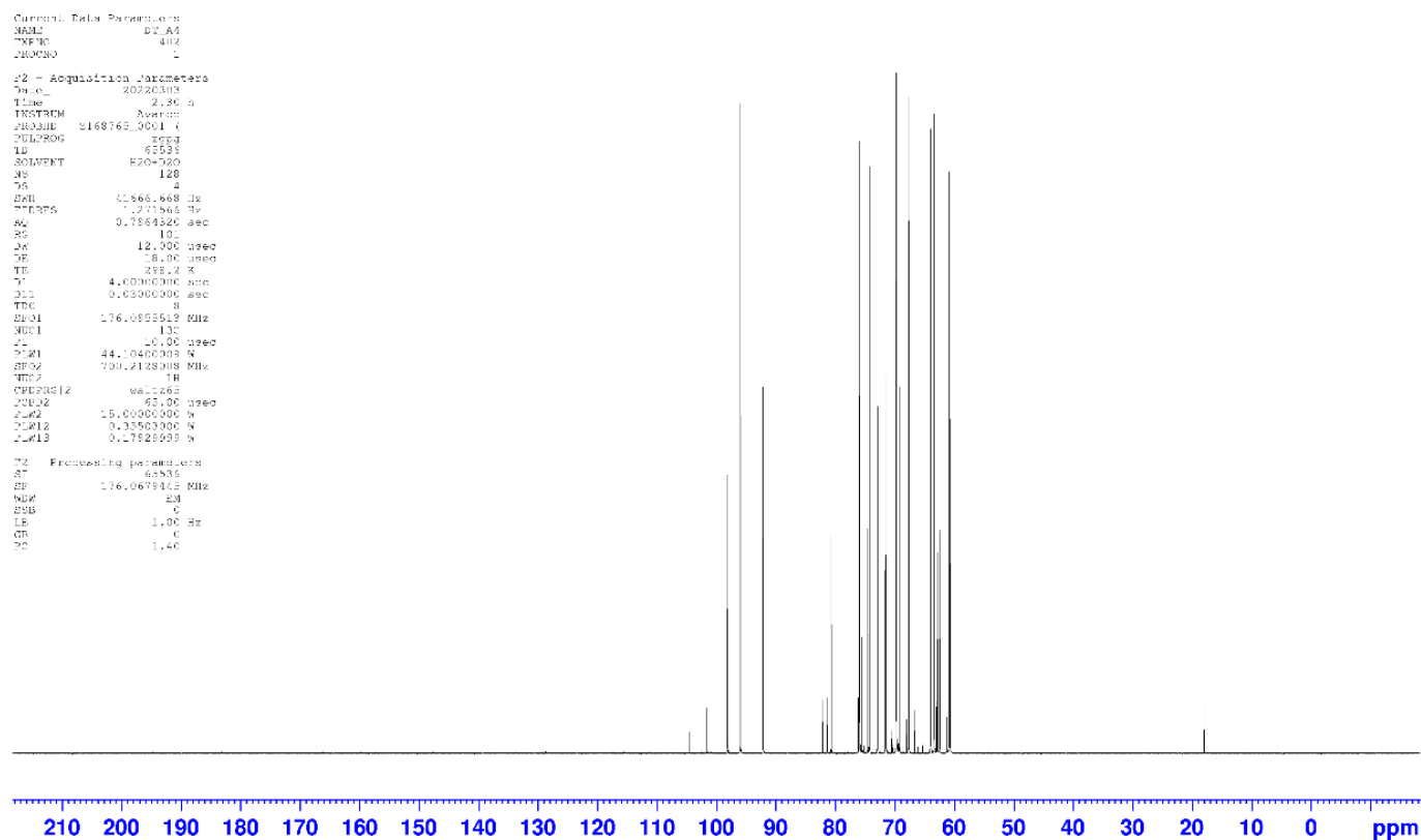
Figure S4 13 C-NMR Fingerprint
