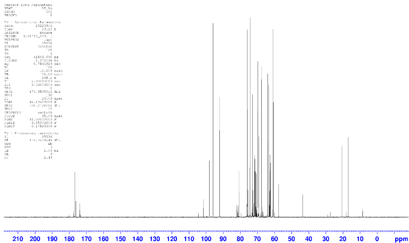
Figure S6 ^{13}\text{C} -NMR Fingerprint
