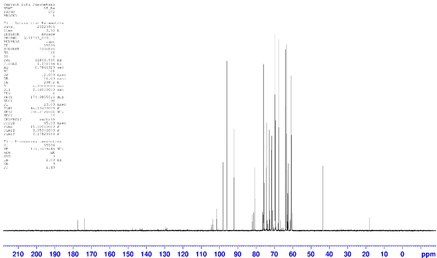
Figure S11 13 C-NMR Fingerprint
