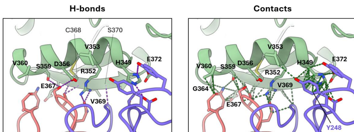
Figure S1: Hydrogen bonds and residue-residue contacts between Tf (green) and TbTfR (pink+blue) in the first binding region.
