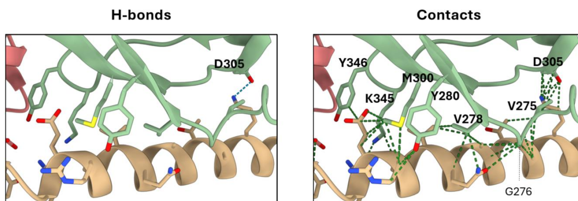
Figure S5: Hydrogen bonds and residue-residue contacts between Hp (green) and HpHbR (gold).
