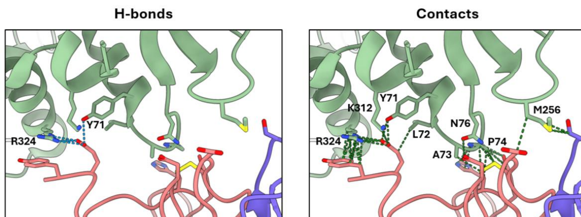
Figure S2: Hydrogen bonds and residue-residue contacts between Tf (green) and TbTfR (pink+blue) in the second binding region.
