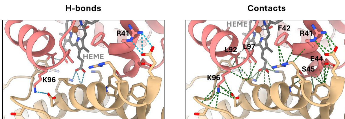
Figure S4: Hydrogen bonds and residue-residue contacts between holo- \beta Hb (pink) and HpHbR (gold).
