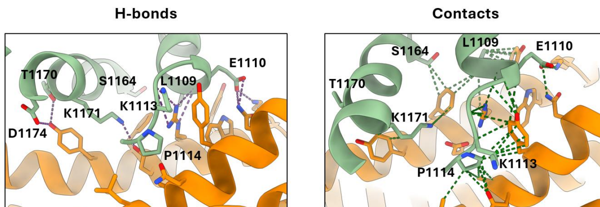
Figure S3: Hydrogen bonds and residue-residue contacts between C3d (green) and ISG65 (orange).
