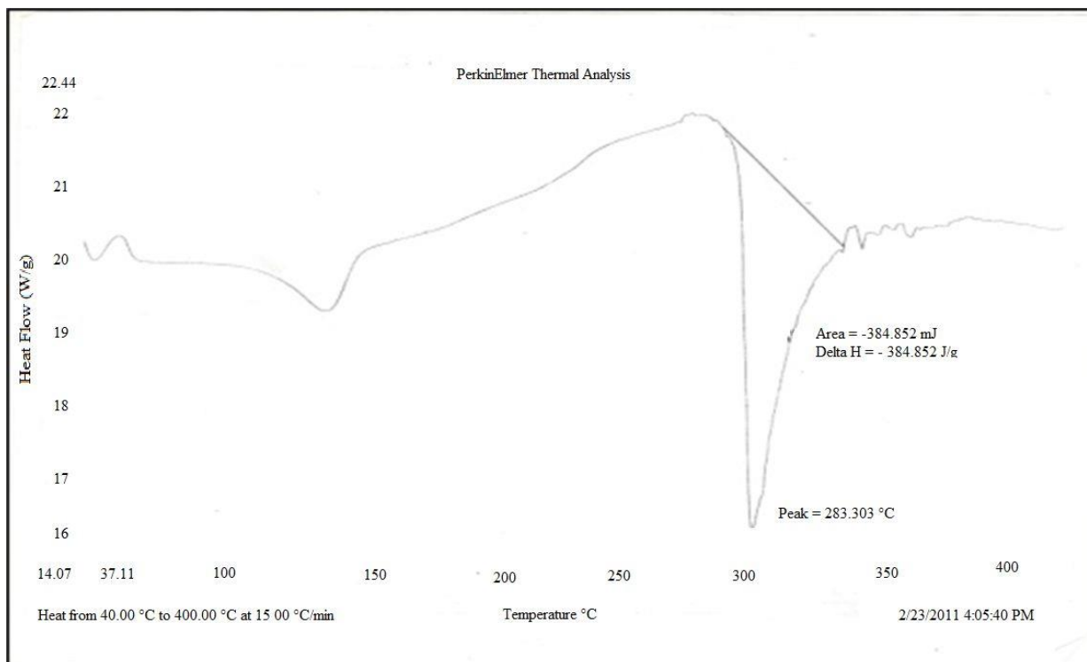
Figure S1. DSC thermogram of isolated hydnocarpic acid
