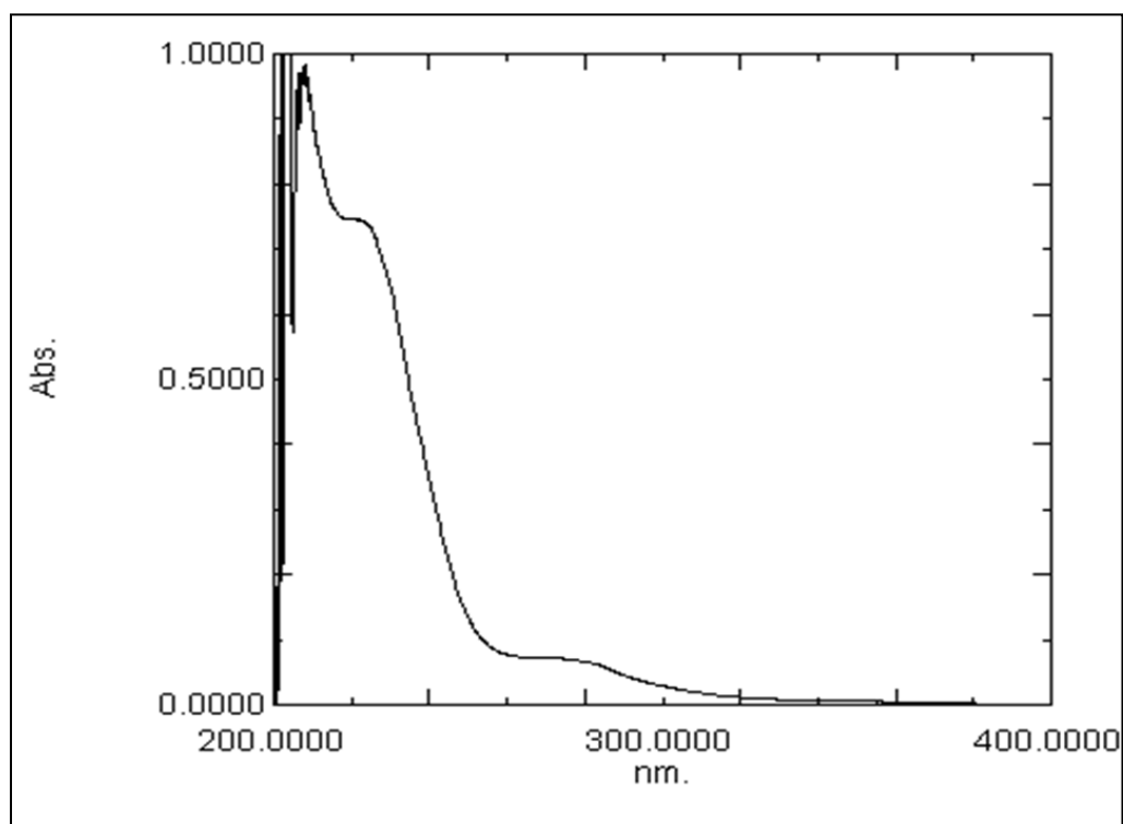
Figure S4. UV spectrum of isolated hydnocarpic acid
