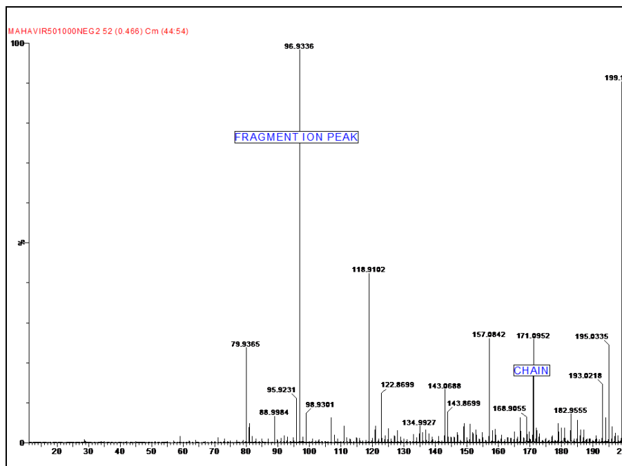
Figure S5. Mass spectra of isolated hydnocarpic acid in positive mode and negative mode
