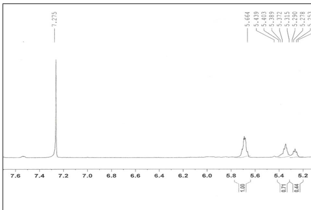
Figure S2. ^1\text{H} NMR spectra of hydnocarpic acid
