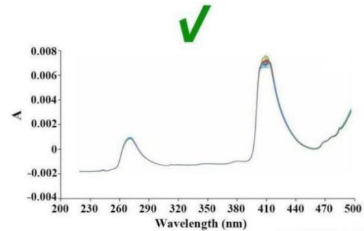
Figure 1. Absorbion spectrum of compound B. A: absorbance.
