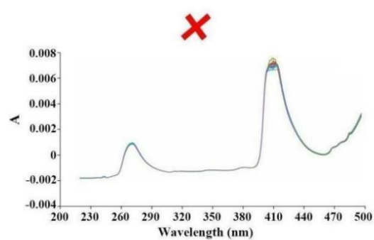
Figure 1. Absorbion spectrum of compound B
